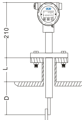
Insertion Type
